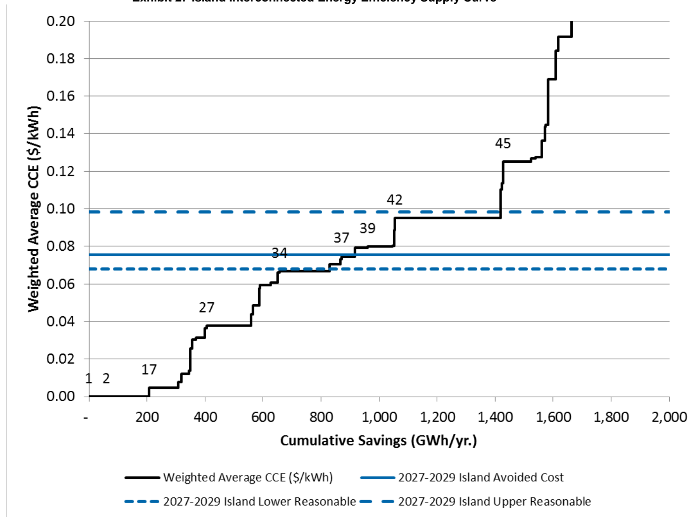
Exhibit 27 Island Interconnected Energy Efficiency Supply Curve
