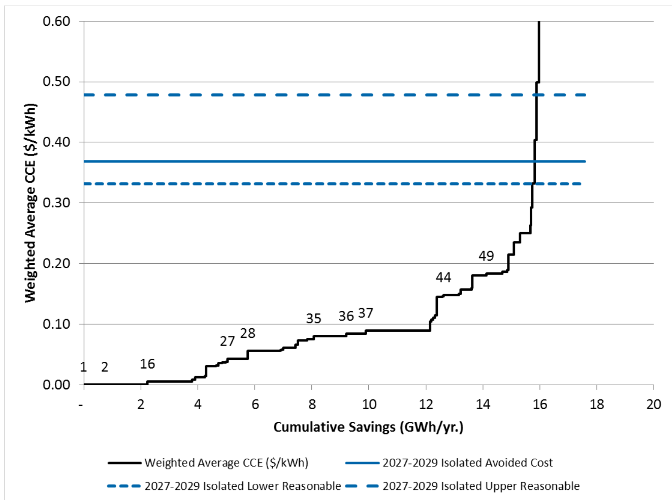
Exhibit 31 Isolated Energy Efficiency Supply Curve
