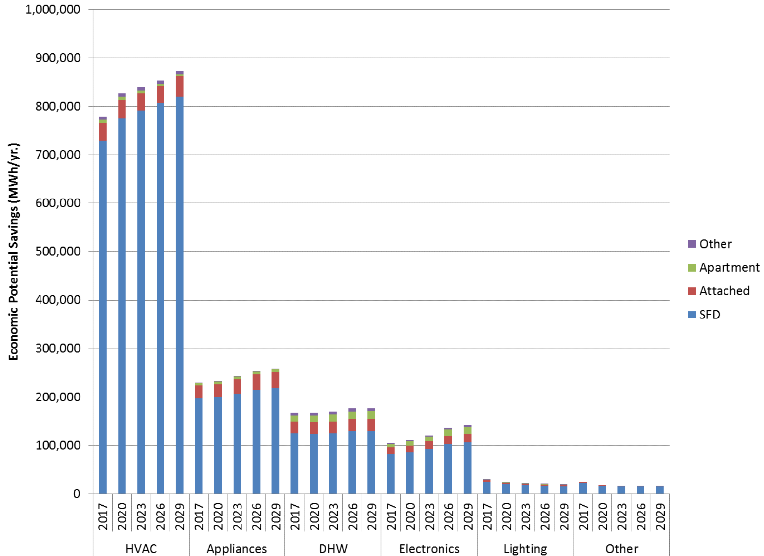
Exhibit 46 Economic Potential Savings by Major End Use, Year and Dwelling Type (MWh/yr.)
