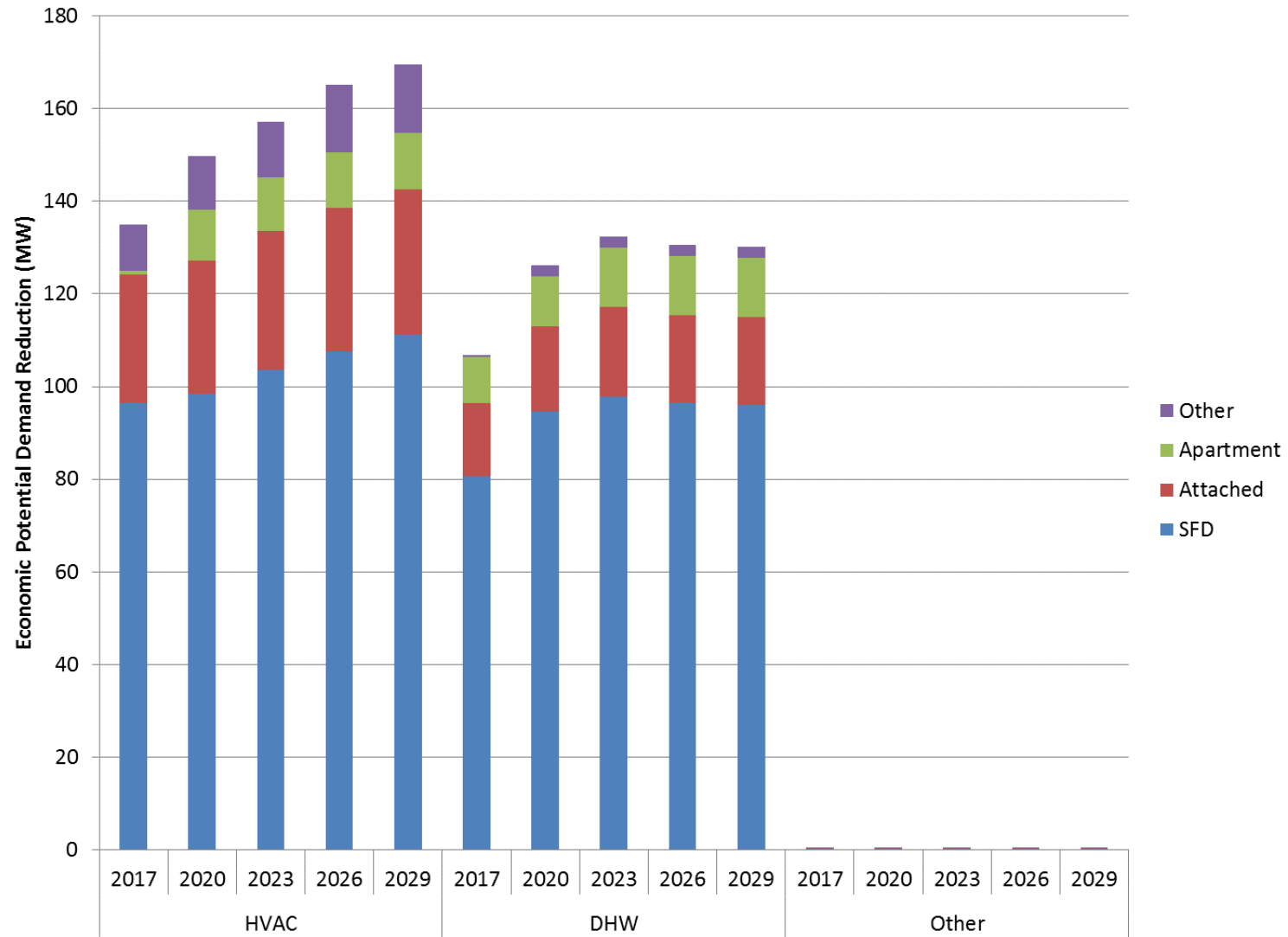
Exhibit 56 Economic Potential Peak Demand Reduction by Major End Use, Year and Dwelling Type (MW)
