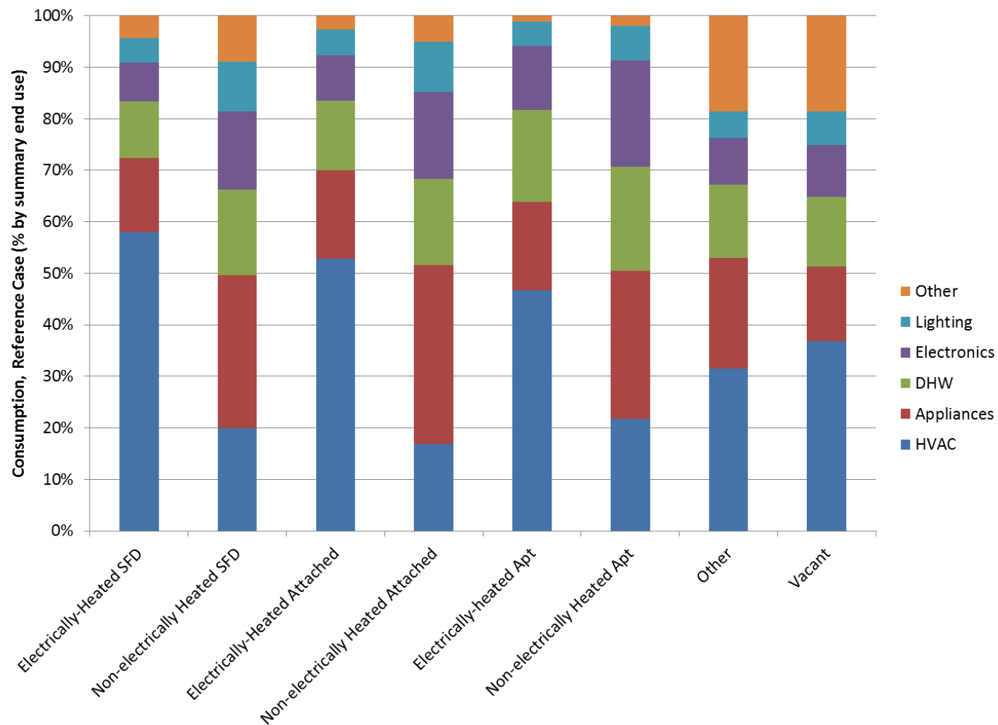
Exhibit 11 Distribution of Electricity Consumption, by Dwelling Type and End Use in the Base Year (2014)
