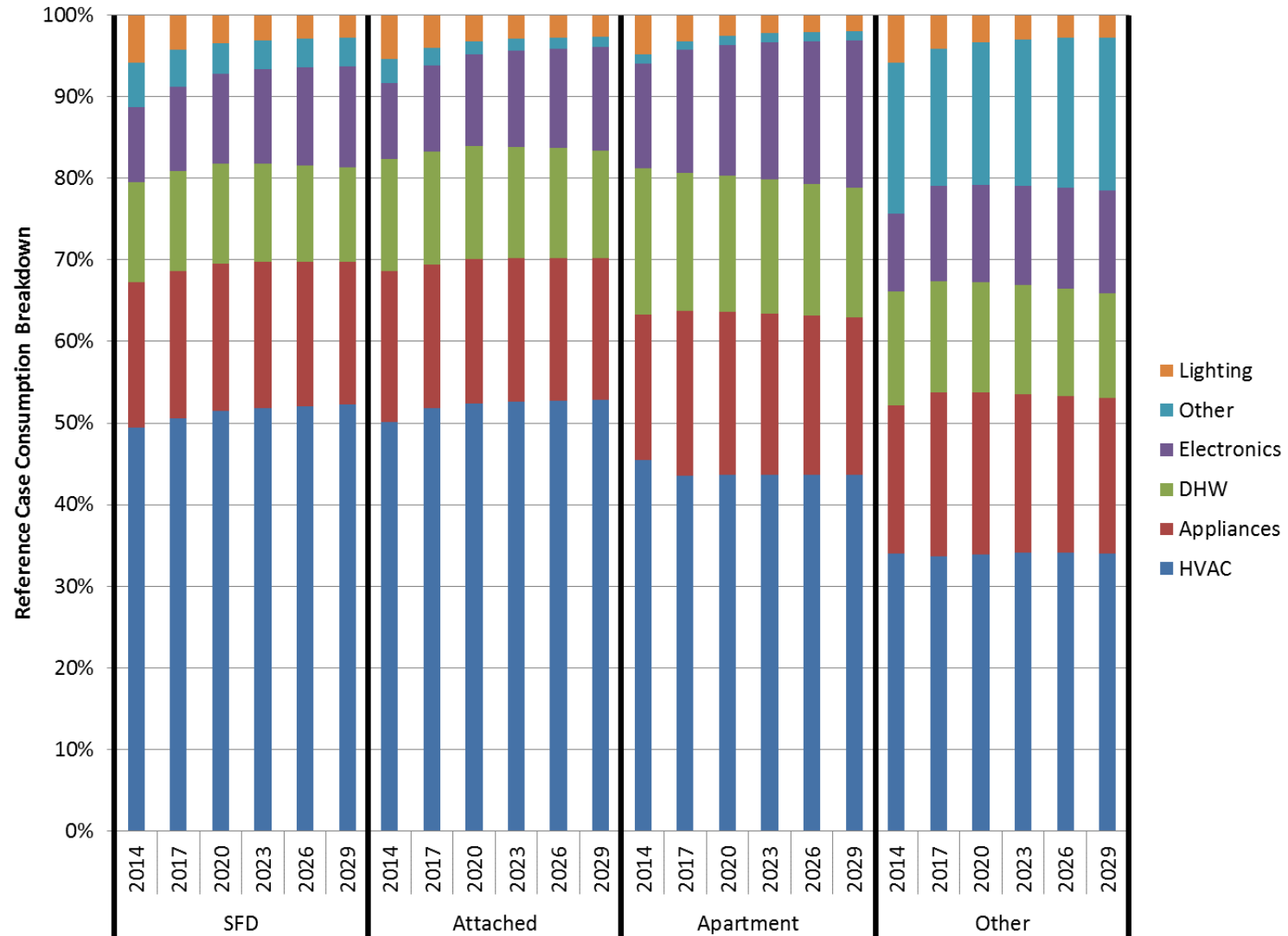
Exhibit 20 Distribution of Electricity Consumption, by Dwelling Type and End Use, Trends to 2029
